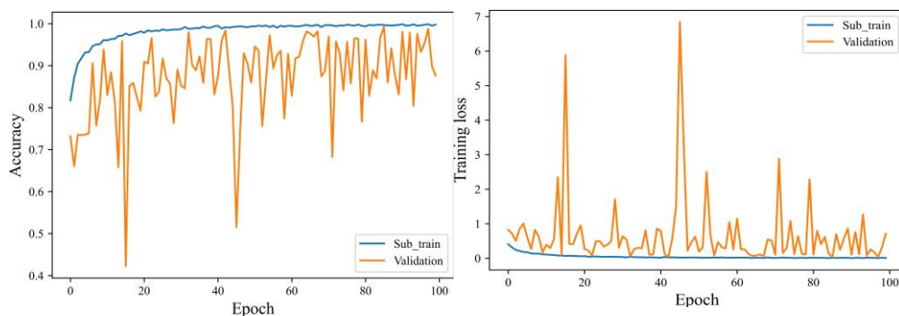
Fig. 3. Training process on server side.
