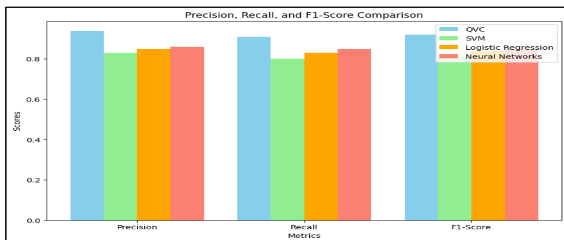
Figure 3: Precision, Recall, and F1-Score Comparison
