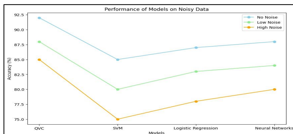
Figure 4: Performance of Models on Noisy Data
