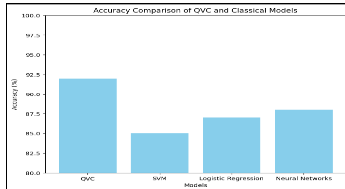
Figure 2: Accuracy Comparison of QVC and Classical Models
